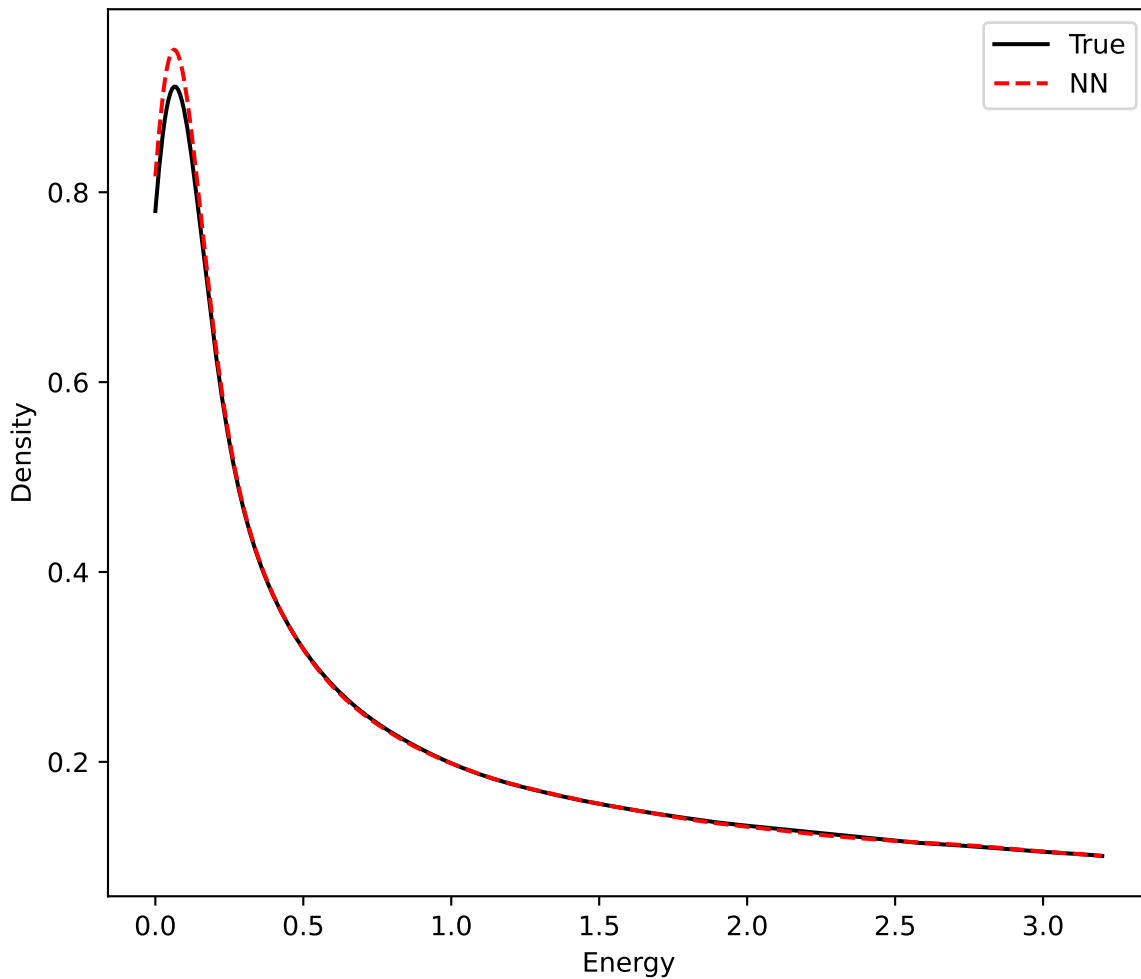
TKE Density Comparison with KS: 0.0083, p-value: 4.6e-93
